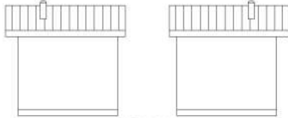
REAR ELEVATION - 2
