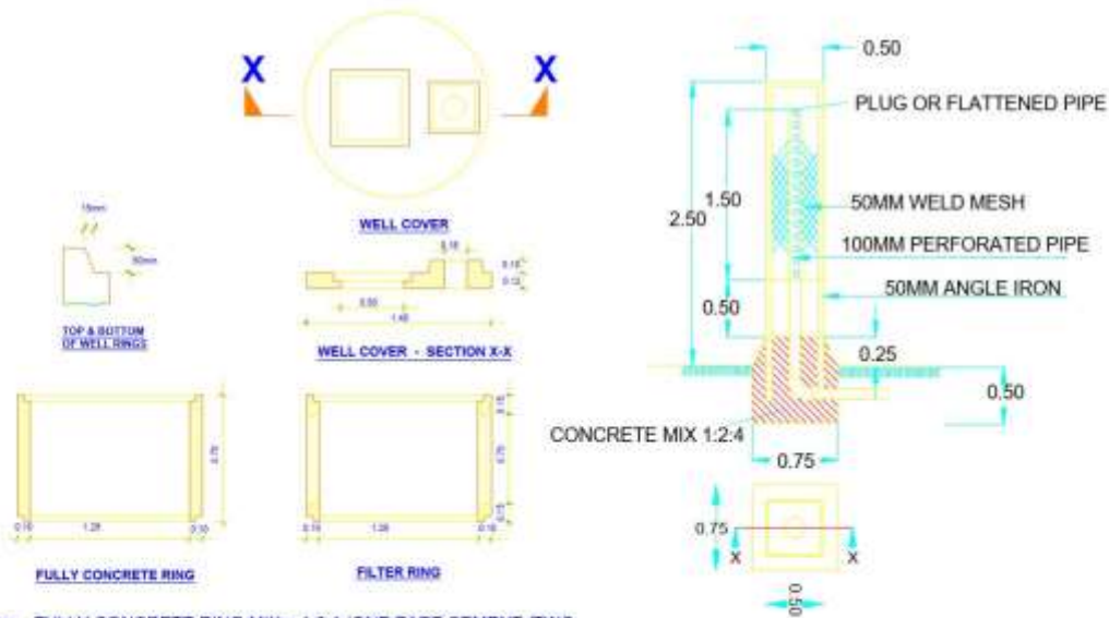
DUG WELL SECTION
